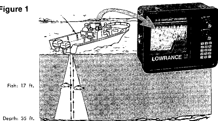
TRULINE RECORDER BOTH SEND AND RECEIVES SIGNALS. RECEIVED SIGNALS ARE INDICATED ON GRAPH PAPER.
